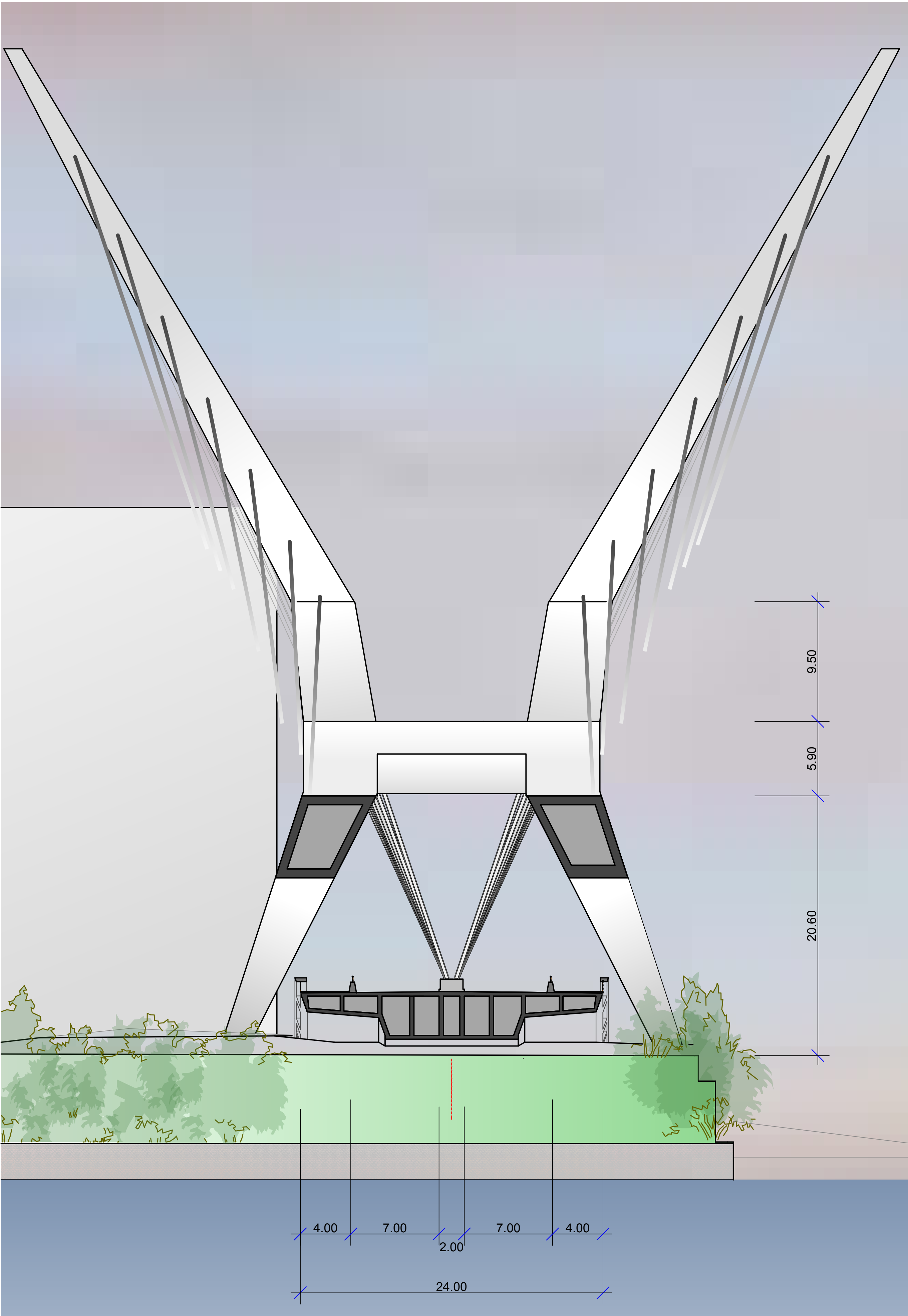
CROSS SECTION
